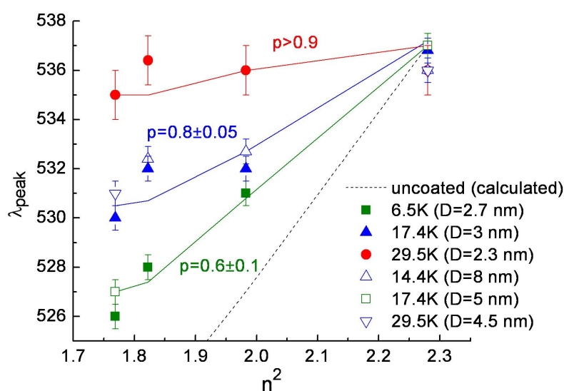
Figure 4.11: Plasmon peak position versus solvent dielectric constant for Au-PNIPAM nanoparticles. The solid lines are theoretical curves calculated using Mie core-shell model. The dotted line is calculated for bare particles (slope = 2).
