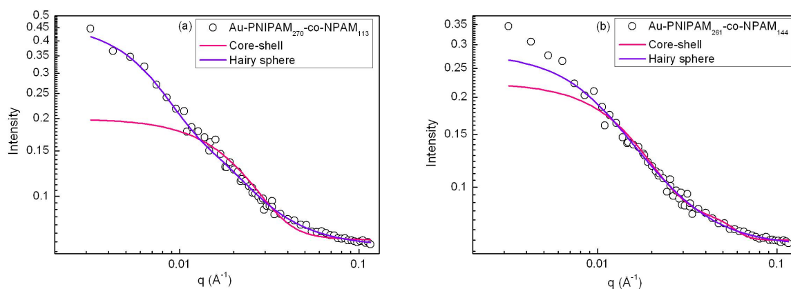
Figure 3.10: The core-shell and hairy sphere adjustments made on the: (a) Au-PNIPAM 270 -co-NPAM 113 scattering curve in absence of salt ( R_g = 6.8 nm) and (b) Au-PNIPAM 261 -co-NPAM 144 scattering curve in presence of salt ( R_g = 7.5 nm) at 20°C.
