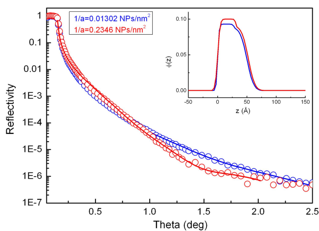
Figure 5.22: X-ray reflectivity curves of Au-PNIPAM 118 -PS 28 thin film at two different surface compressions (150 mM NaCl, T = 20°C); the solid lines are theoretical best-fit curves with corresponding gold core concentration profiles shown in the inset.
