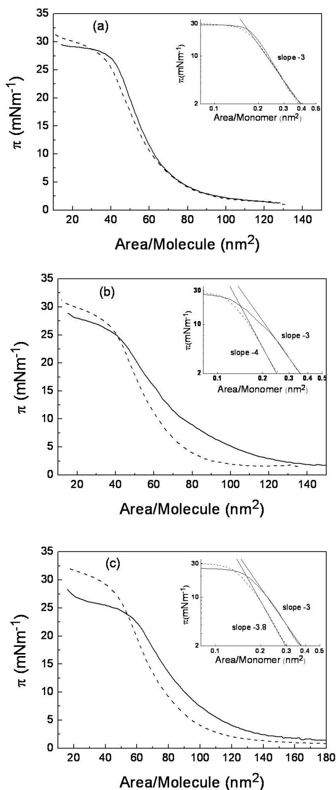
Figure 5.3: Compression isotherms of (a) Cpa-PNIPAM 265 at T= 20°C(solid line), T= 33°C (dashed line); (b) Cpa-PNIPAM 270 -co-NPAM 113 at T= 20°C (solid line), T= 30°C (dashed line); (c) Cpa-PNIPAM 261 -co-NPAM 144 at T= 20°C (solid line), T= 29°C (dashed line). The insets show double logarithmic plots with calculated slopes for comparison (straight lines).
