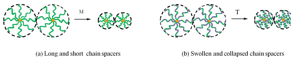
Figure 5.8: Control of interparticle distance d in: (a) Au-PNIPAM monolayer with PNIPAM molecular mass and (b) Au-PNIPAM-co-NPAM monolayer with temperature.
