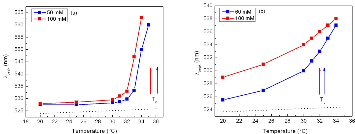
Figure 4.18: Position of SPR peak as a function of temperature for: (a) Au-PNIPAM 127 and (b) Au-PNIPAM 270-co-NPAM 113 dispersed in 50 - 60 (blue) and 100 mM (red) NaCl solutions. The T_c for free chains at the corresponding NaCl concentrations are indicated by vertical arrows. The black dotted lines represent the evolution with temperature of SPR peak position in water.
