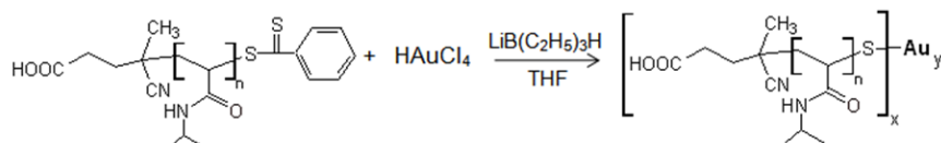
Figure 2.10: The synthesis route of Cpa-PNIPAM-protected gold nanoparticles
