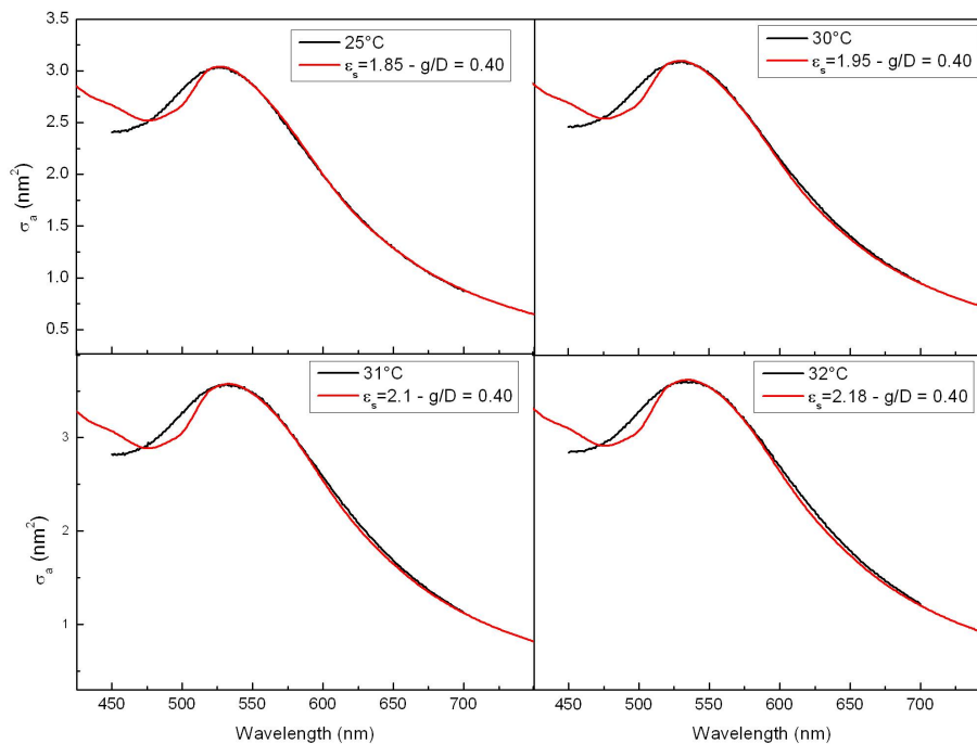
Figure 4.21: Fits of extinction spectra of Au-PNIPAM 270 -co-NPAM 113 particles dispersed in 60 mM NaCl at varying temperatures.
