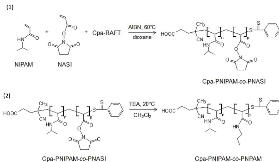
Figure 2.4: Schematic representation of reaction routes for: (1) copolymerization of Cpa-PNIPAM-NASI (1) and, (2) conversion of Cpa-PNIPAM-co-NASI to Cpa-PNIPAM-co-NPAM by aminolysis using n -propylamine.
