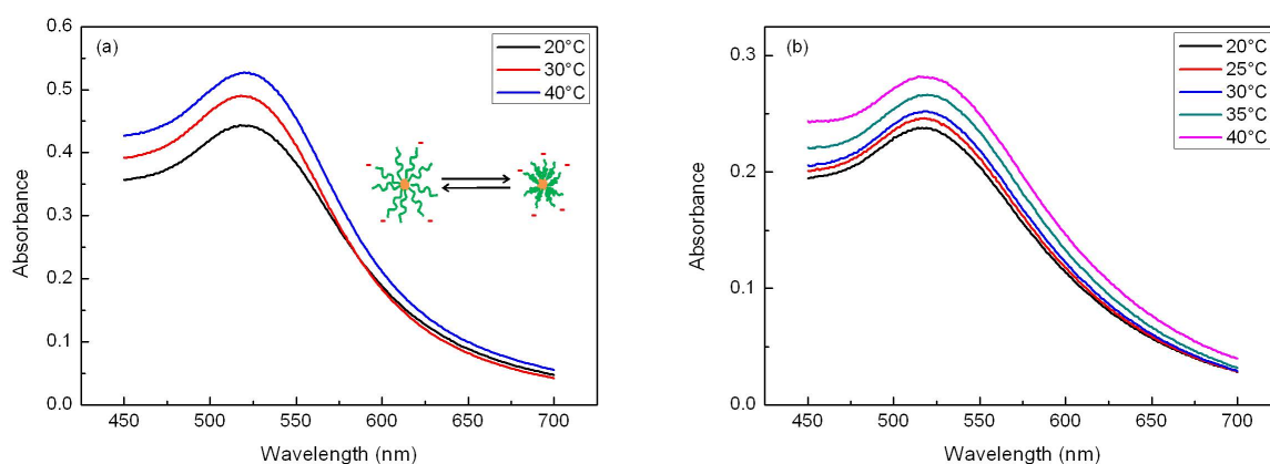
Figure 4.15: UV-vis absorption spectra as a function of temperature: (a) Au-PNIPAM 127 and (b) Au-PNIPAM 270-co-NPAM113 dispersed in water.
