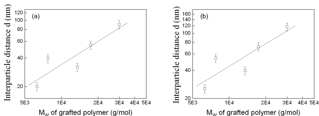
Figure 5.6: Interspace distance versus graft polymer chain length evaluated from: (a) A_{p\text{-loop}} and (b) A_{p\text{-pancake}} ; the solid lines are best-fit curves with slopes of 0.80 and 0.81, respectively.
